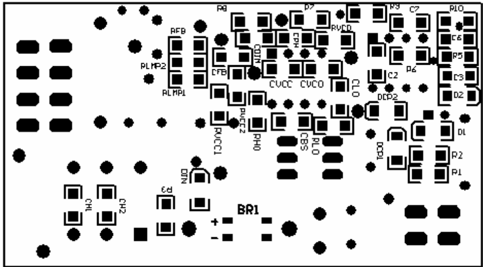
Bottom Assembly
